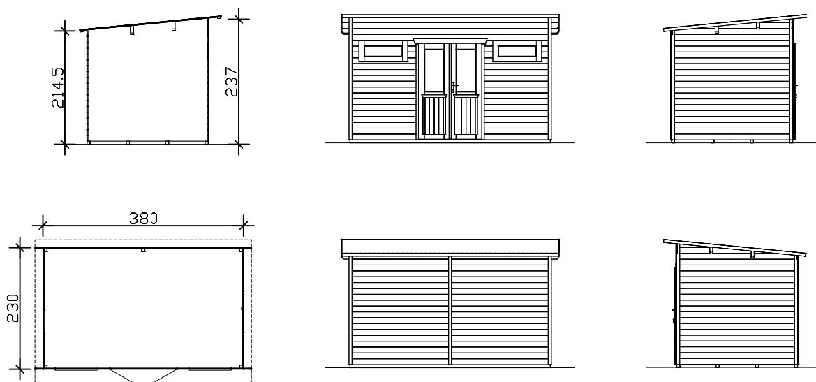
Floor plan, cross-section and elevations M 1:100
