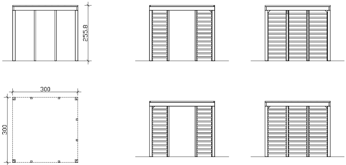
Floor plan, cross-section and elevations M 1:100
